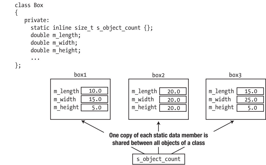
Figure 12-6. Static class members are shared between objects
