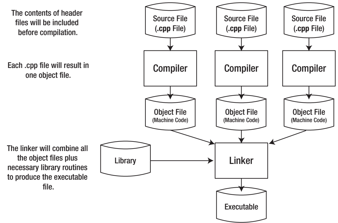
Figure 1-1. The compile and link process
