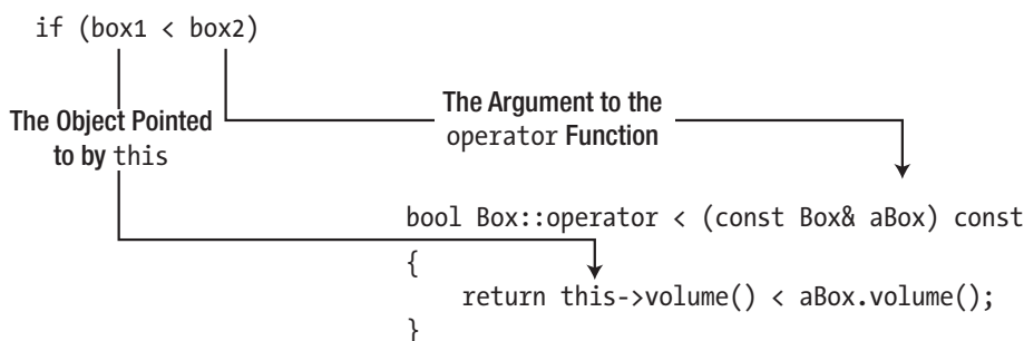
Figure 13-1. Overloading the less-than operator
