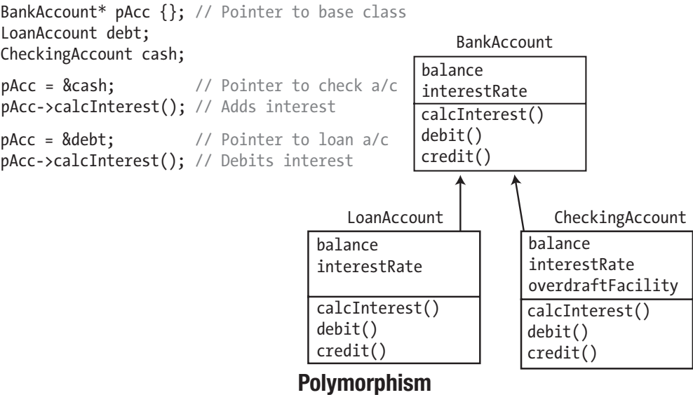
Figure 12-5. An example of polymorphism
