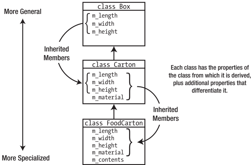
Figure 14-1. Classes in a hierarchy
