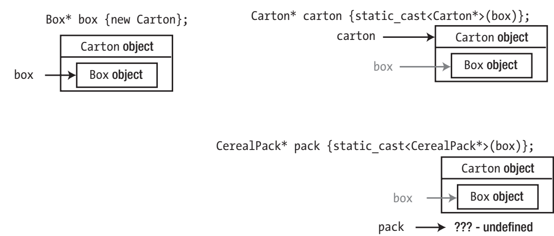
Figure 15-5. Casting pointers down a class hierarchy
