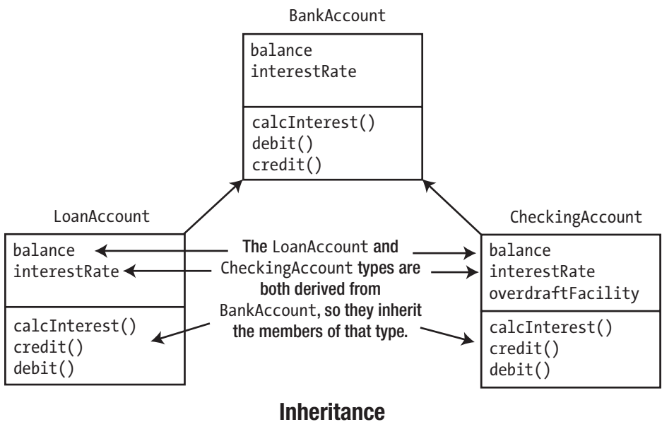
Figure 12-4. An example of inheritance
