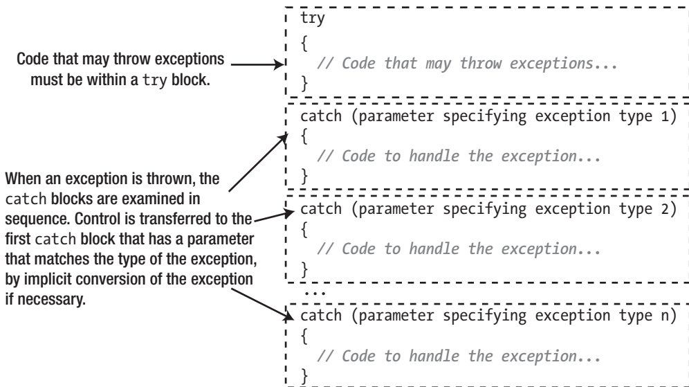
Figure 16-1. A try block and its catch blocks
