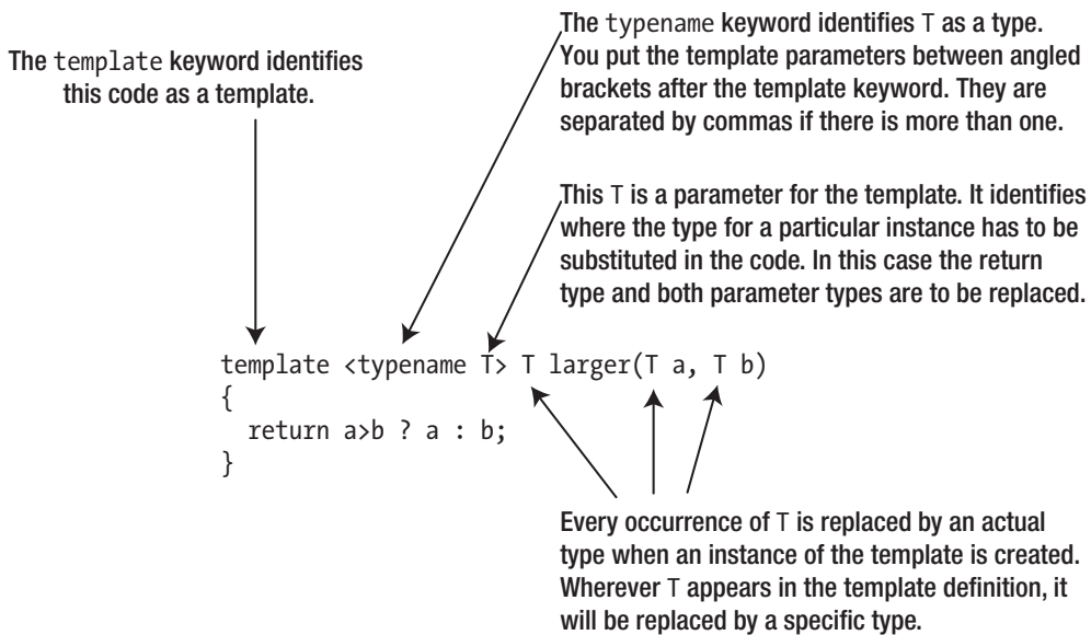
Figure 10-1. A simple function template
