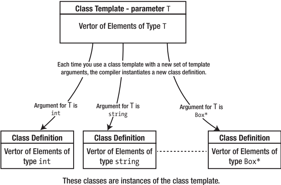
Figure 17-1. Class template instantiation
